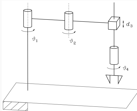
Figure 1: RRPR manipulator.
